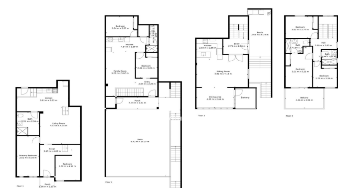
TOTAL: 335 m 2 BELOW GROUND: 81 m 2 , FLOOR 2: 59 m 2 , FLOOR 3: 42 m 2 , FLOOR 4: 53 m 2 EXCLUDED AREAS: PORCH: 25 m 2 , PATIO: 67 m 2 , LOW CEILING: 11 m 2 , BALCONY: 21 m 2
